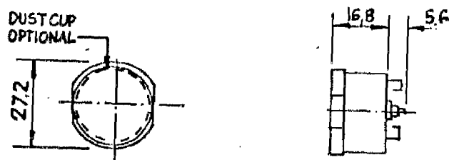
TYPE FA FLUSH MOUNT SOLDER LUGS AUTO-RESET
