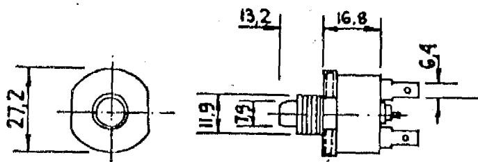
TYPE FPM PANEL MOUNT QUICK CONNECT MANUAL RESET
