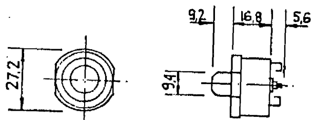
TYPE FM FLUSH MOUNT SOLDER LUGS MANUAL RESET
