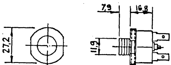
TYPE FPA PANEL MOUNT QUICK CONNECT AUTO-RESET
