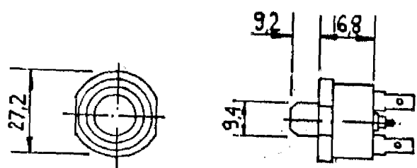
TYPE FM FLUSH MOUNT SOLDER LUGS MANUAL RESET
