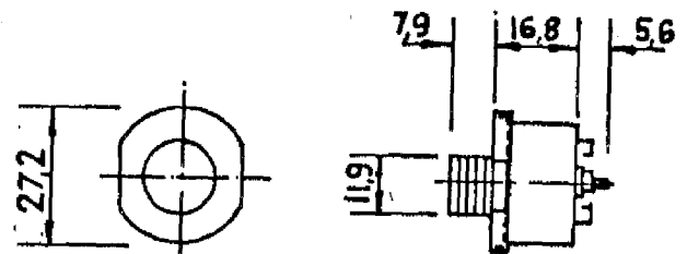
TYPE FPA PANEL MOUNT SOLDER LUGS AUTO-RESET
