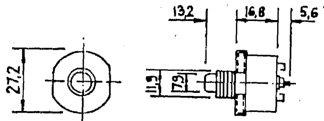
TYPE FPM PANEL MOUNT SOLDER LUGS MANUAL RESET
