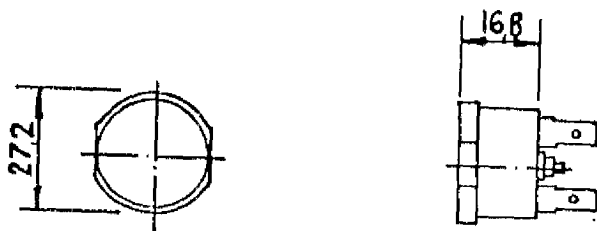
TYPE FA FLUSH MOUNT QUICK CONNECT AUTO-RESET
